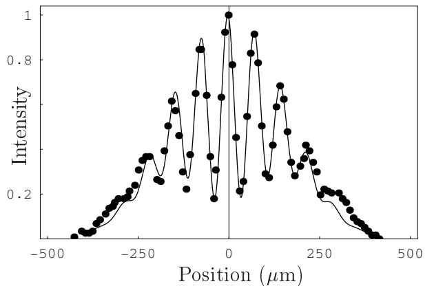
Figure 1: Comparison between theoretical prediction derived here (solid line) and experimental data taken from [1] (solid circles) for neutron double-slit diffraction.
